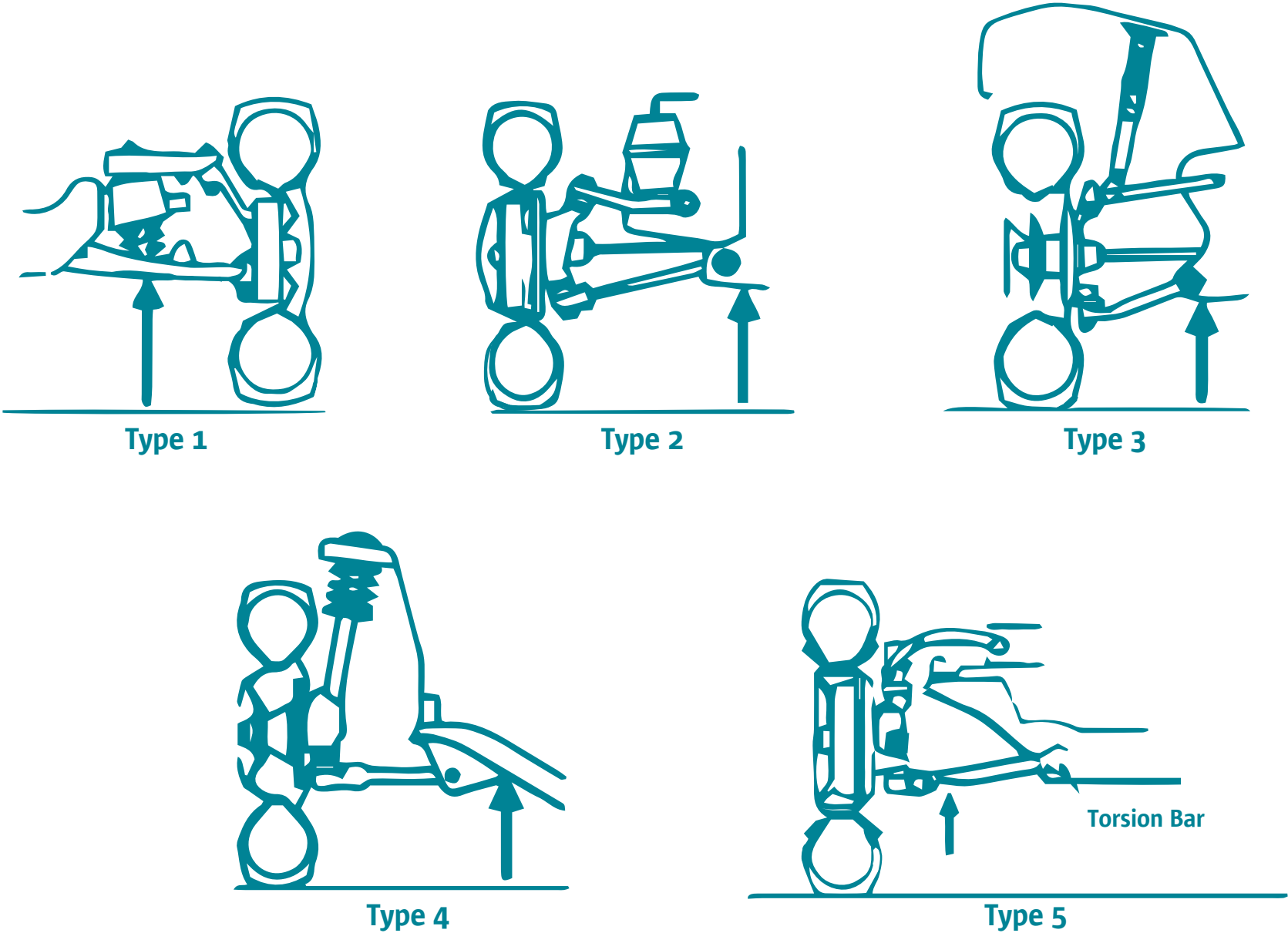
Figure 2. Suspension Types
