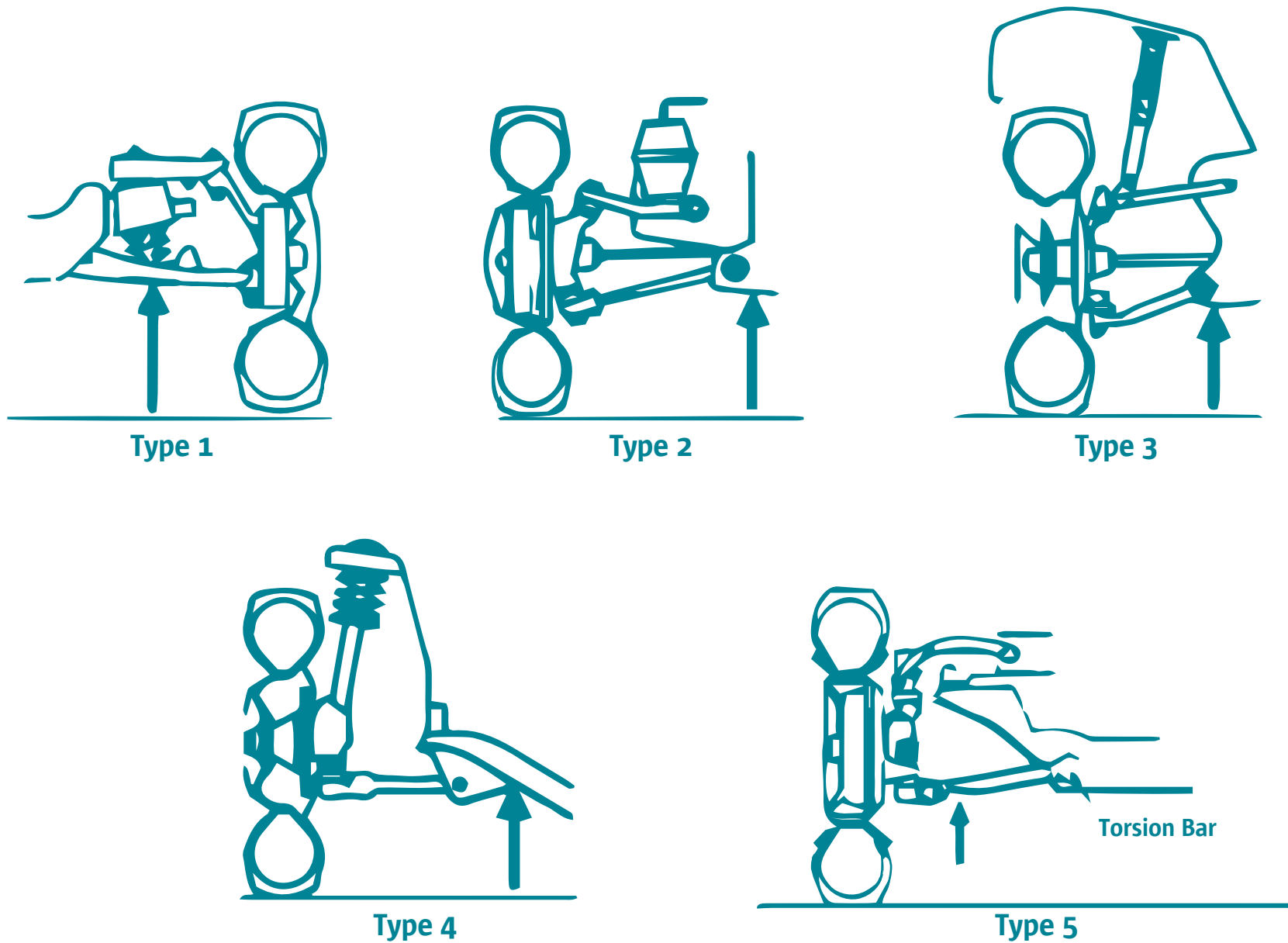
Figure 2. Suspension Types
