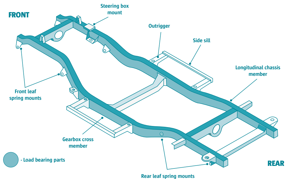
Figure 1. Primary structural components
